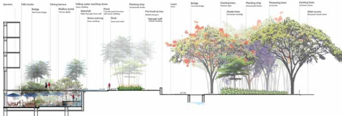
Section - waterfall pond and central pond NTS
